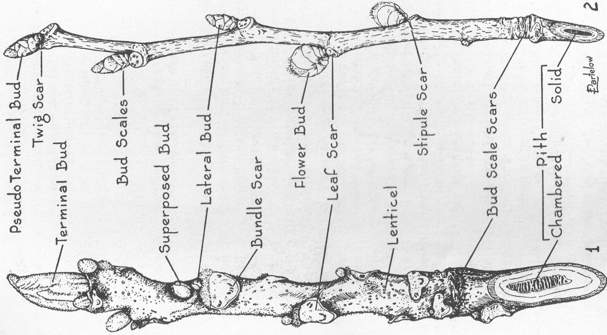
PLATE 8.—Twig details of (1) butternut, (2) elm.
